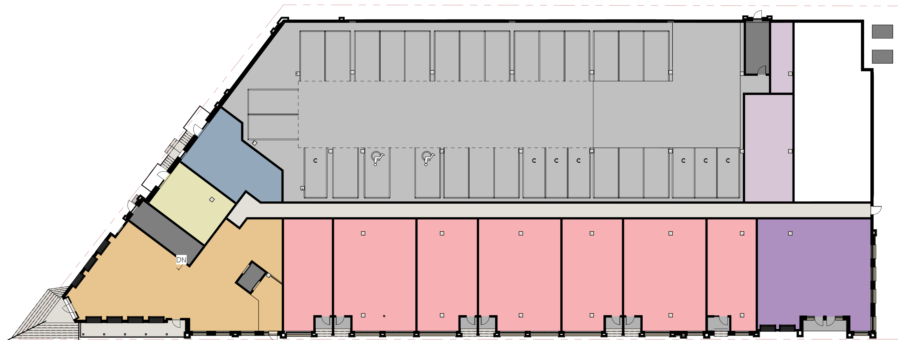
1ST FLOOR PLAN 1" = 20'-0"
